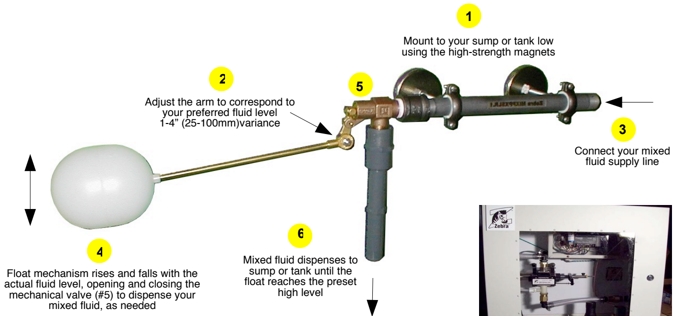
Zebra Fill-Station, using Zebra Proportioning Pump
