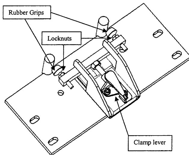
Fig 3: Adjustment
