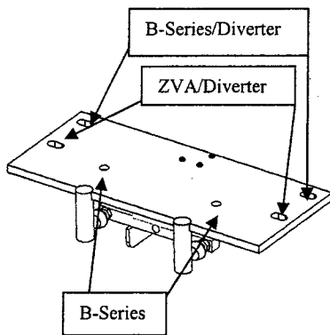
Fig 2: Mounting Holes
